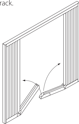
Bi-parting Sash Folding Bottom Track Option
